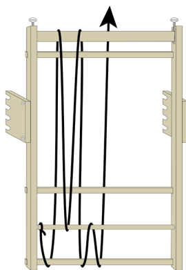
WARPING PATH 7
