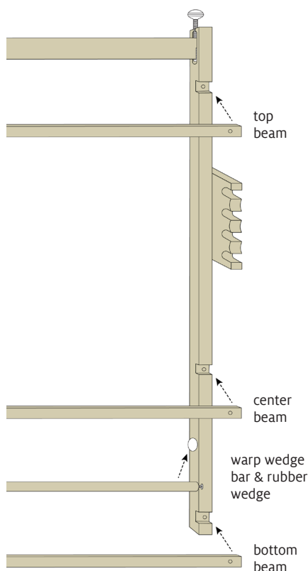
FIGURE 3: ATTACH BARS
