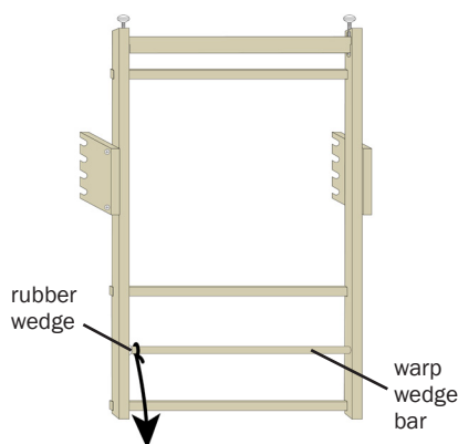
WARPING PATH 1
