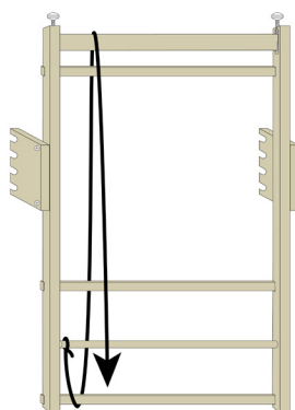
WARPING PATH 3
