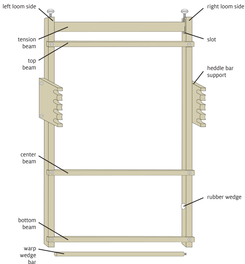
FIGURE 1: PARTS OF THE TAPESTRY LOOM
