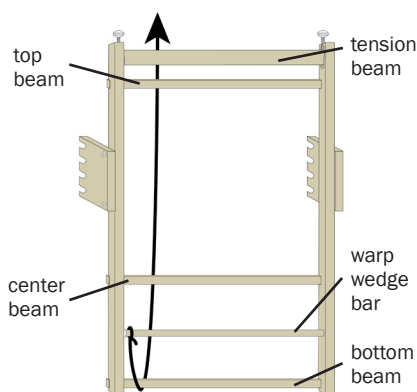
WARPING PATH 2
