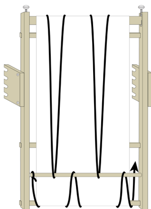
WARPING PATH 7
