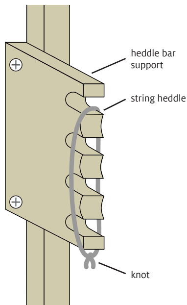
FIGURE 4: MEASURING STRING HEDDLES
