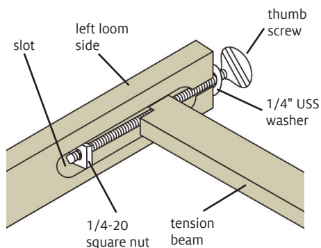
FIGURE 2: INSTALL TENSION BEAM
