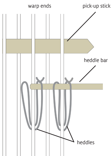
FIGURE 5: INSTALLING HEDDLES
