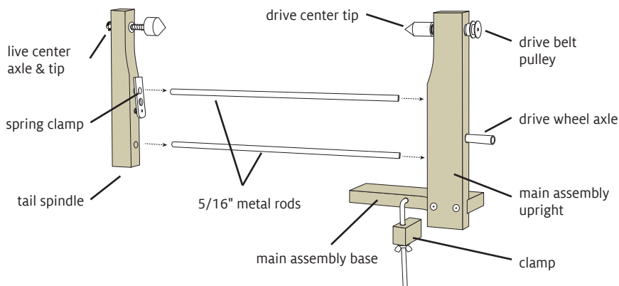
FIGURE 1: INSTALL TAIL SPINDLE (DOUBLE END WINDER ONLY)
