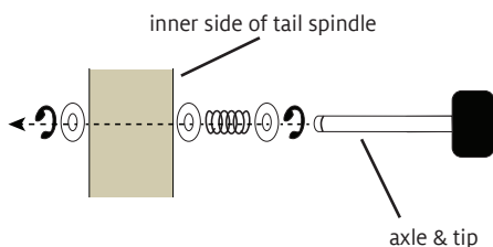
FIGURE 4: INSTALLING THE LIVE CENTER AXLE AND TIP
