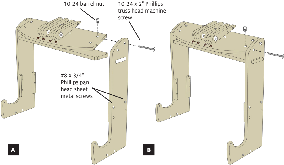
FIGURE 5: ATTACH LEVER BRACE
