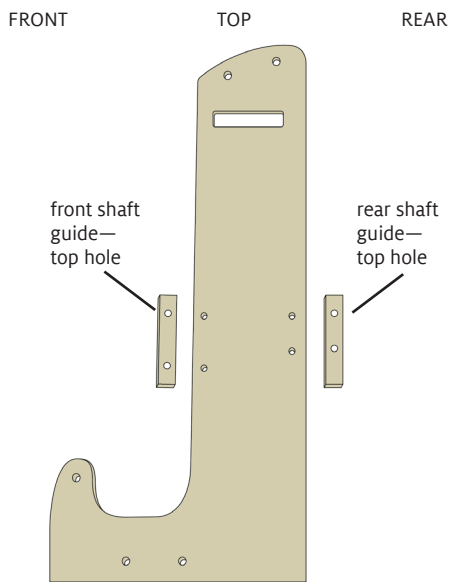
FIGURE 3: CASTLE SIDE AND SHAFT GUIDES
