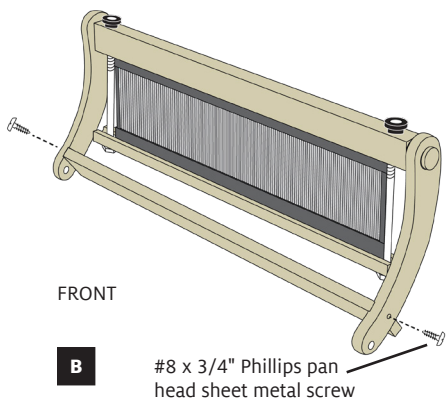
FIGURE 16: INSTALL THE REED
