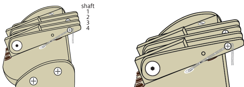
FIGURE 12: CONNECTING LEVER CORDS TO LEVERS
