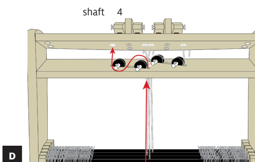
FIGURE 11: FEEDING LEVER CORDS
