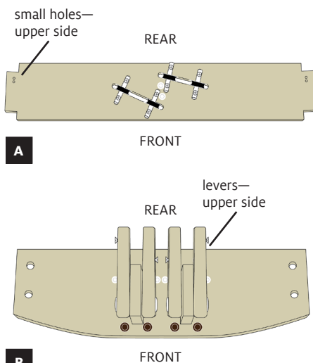
FIGURE 4: ORIENT PULLEY BRACE AND LEVER BRACE
