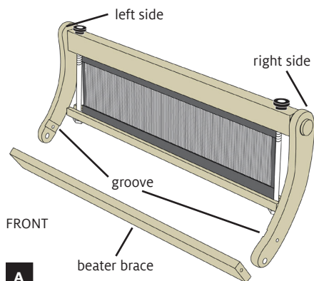
FIGURE 17: ASSEMBLE THE PIVOT BEATER
